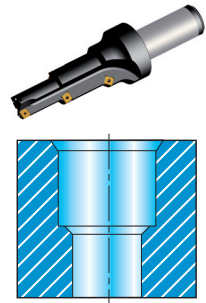
B6. Counterbore with chamfers
