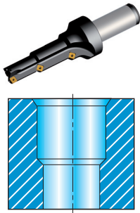
B4. Step and chamfer
