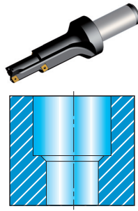
B5. Counterbore and chamfer
